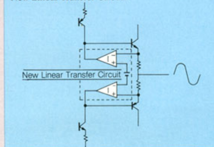
New Linear Transfer Circuit
